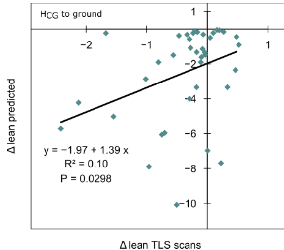
Figure 4.11: Link between lean angle changes ( ^\circ ) predicted by computation of the model from the HCG to the ground and measured from TLS scans.
