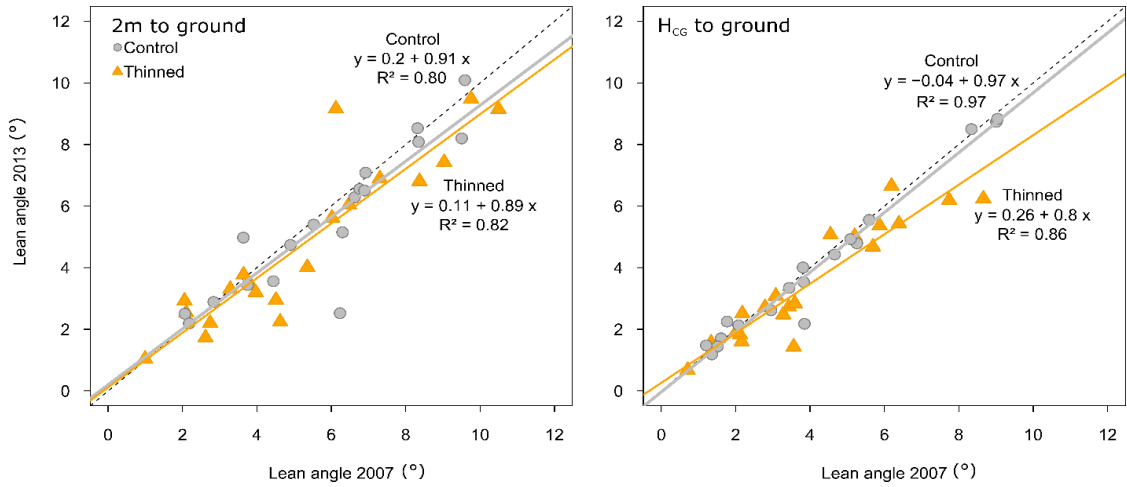
Figure 4.4: Relationship between the stem lean ( ^\circ ) deduced from TLS scans at 2-m height (left) and at the height of the centre of mass (right) in 2007 and 2013 of control and thinned poles.
